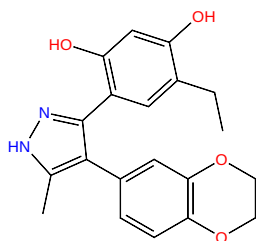
title: Pyrazole Inhibitor 1 (CCT018159) PDB ID Reference: 2BT0 (Not used for docking) FP IC50: 0.28 Reference Papers: (Brough, et al., 2008)
